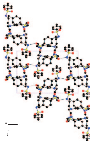
Figure 2. Crystal packing of tstaec .
