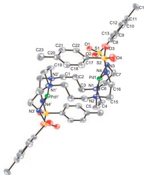
Figure 3. ORTEP drawing of the structure of [Pd_2(tstaec)] \cdot 2CH_3CN showing the 25% probability thermal ellipsoids and atom labeling scheme. Hydrogen atoms are omitted for clarity.
