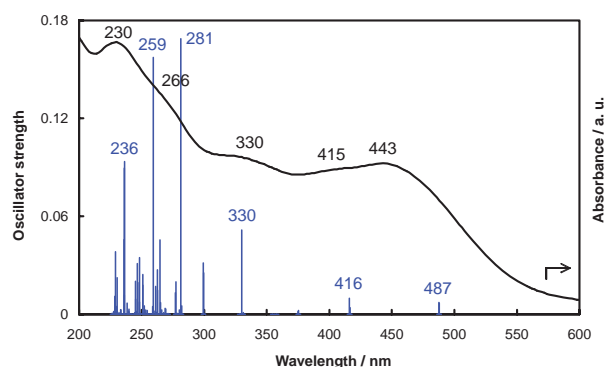
Figure 5. Diffused reflectance spectra of [Pd 2 (tstaec)]·CH 3 CN with the TD-DFT calculated transition energies as absorption wavelengths in nm and oscillator strengths indicated by vertical lines for comparison.
