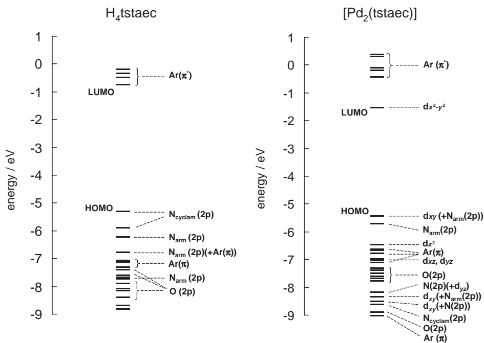
Figure 6. MO energy diagrams for H_4tstaec (left) and [Pd_2(tstaec)] (right).
