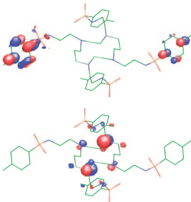
Figure 7. Calculated isosurface of HOMO (bottom) and LUMO (top) for H_4tstaec .
