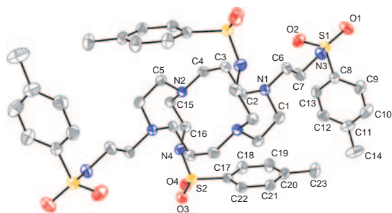
Figure 1. ORTEP drawing of the structure of H_4tstaec showing the 25% probability thermal ellipsoids and atom labeling scheme. Hydrogen atoms are omitted for clarity.
