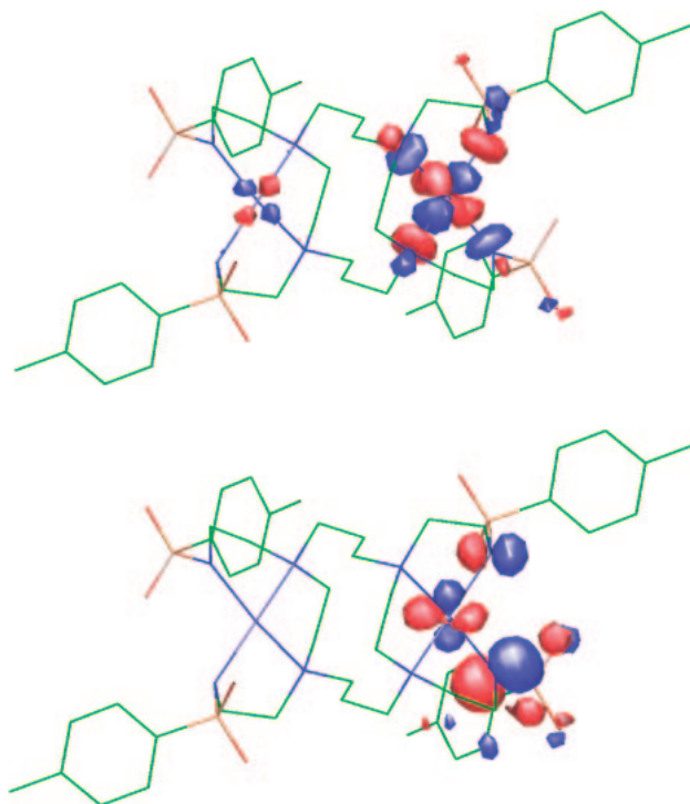
Figure 8. Calculated isosurface of HOMO (bottom) and LUMO (top) for [Pd_2(tstaec)] .
